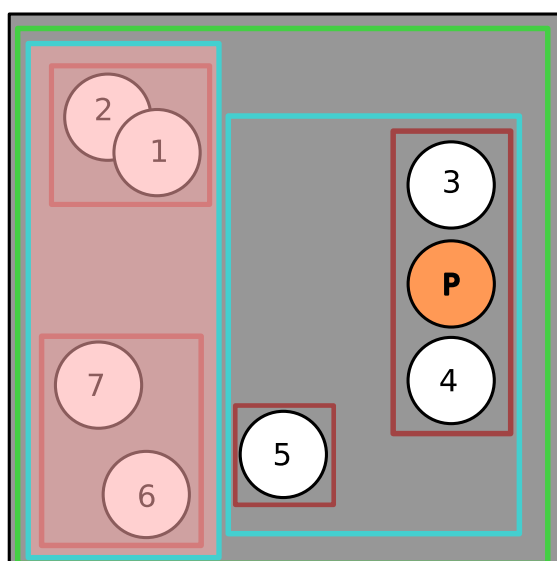
Figure 182: Querying an AABB-tree (1/3)
